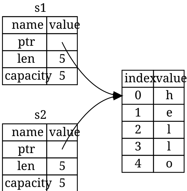
Figure 4-2: The representation in memory of the variable s2 that has a copy of the pointer, length, and capacity of s1
